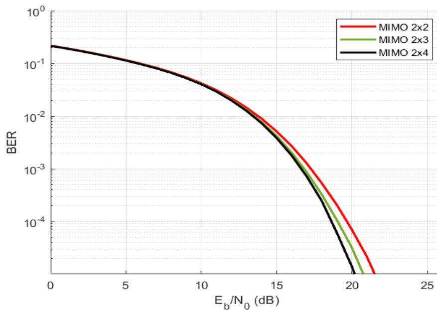
Figure 3: 16 PSK over Rician
