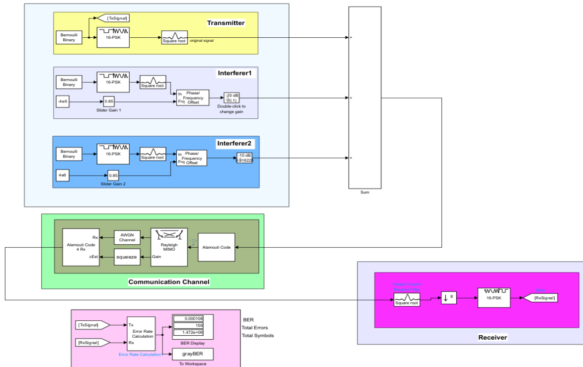
Figure 2: Simulation Model of the Communication System with Interference using 16-PSK
