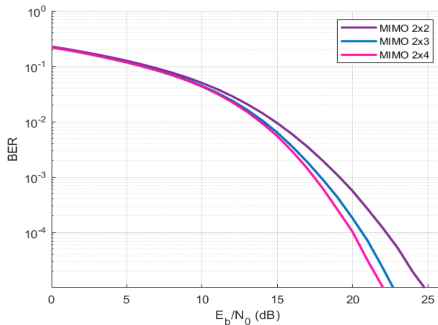
Figure 4: 16 PSK over Rayleigh
