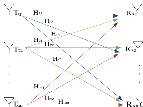
Figure 1: m \times n MIMO System
