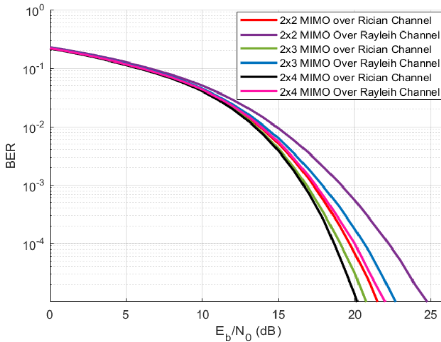
Figure 5: 16 PSK over Rician and Rayleigh
